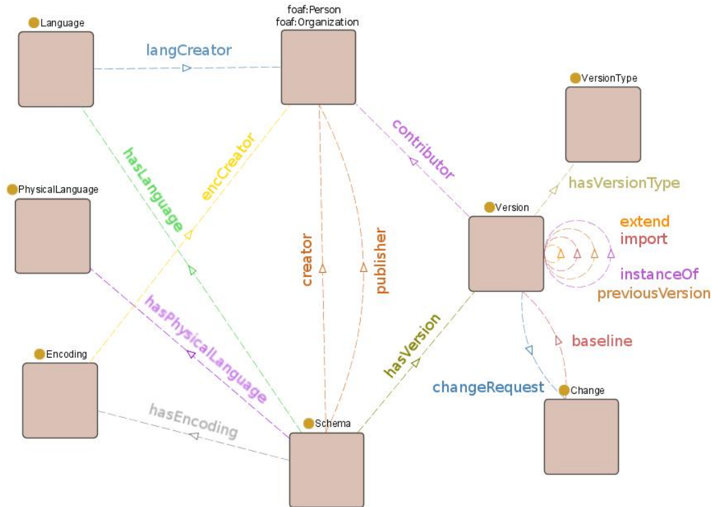
Figure 8: The Ontology Registry Schema
